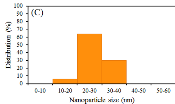
Figure 3. Particle size distribution histogram of \text{WO}_3 nanoparticles (a) before RF plasma, and after RF plasmas of (b) oxygen, (c) nitrogen, and (d) argon.
